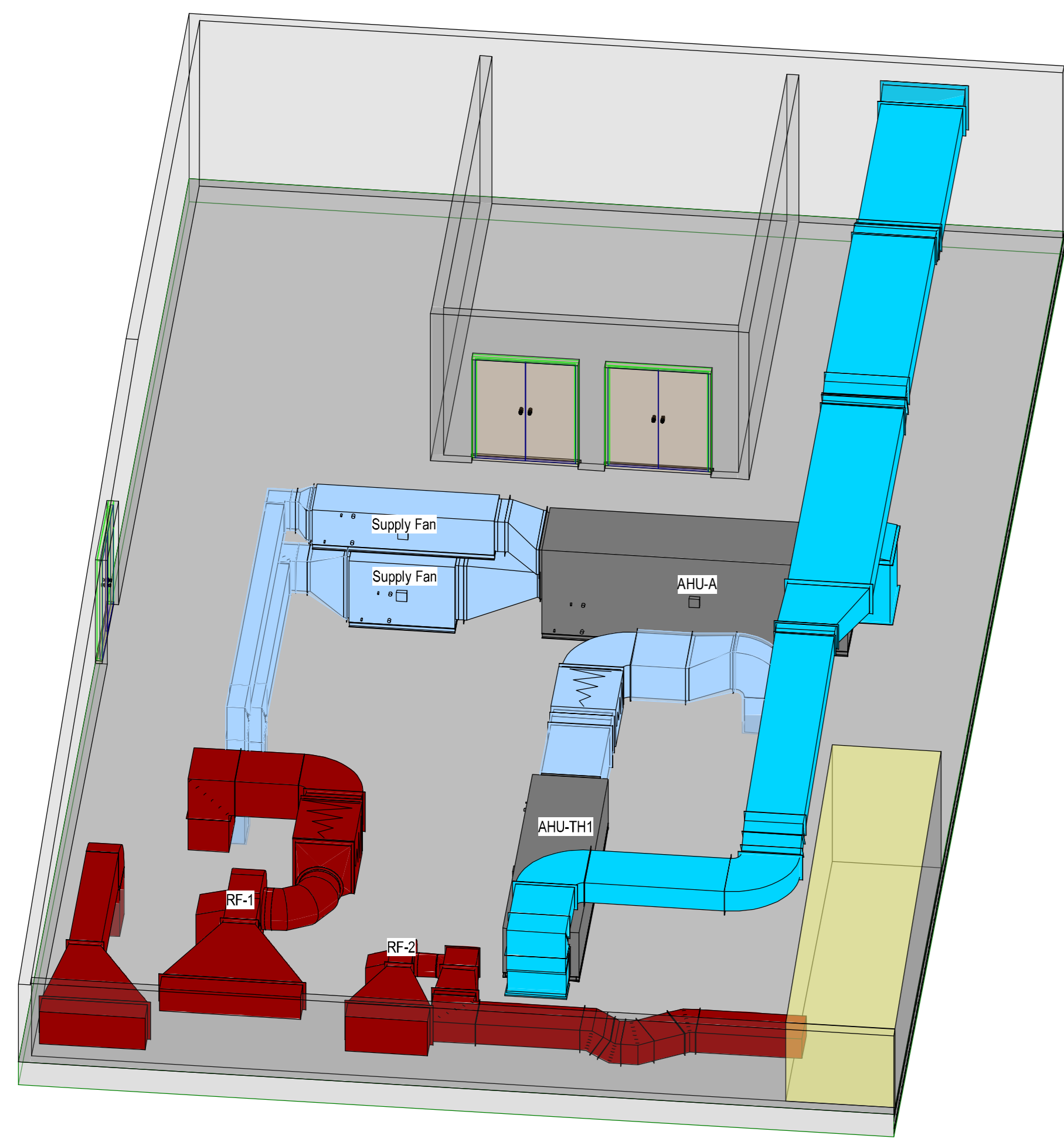
1 Plantroom View 1
