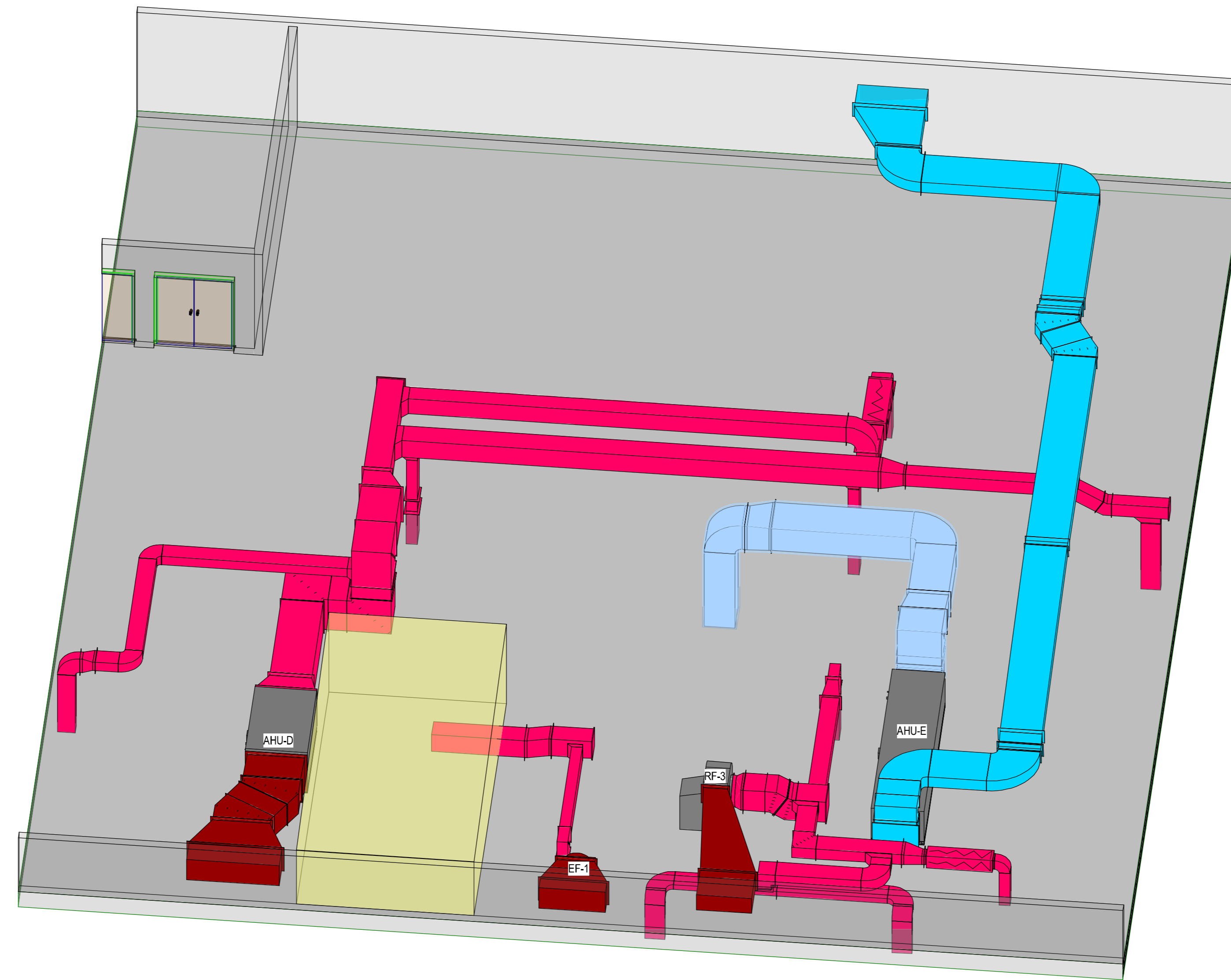
2 Plantroom View 2
