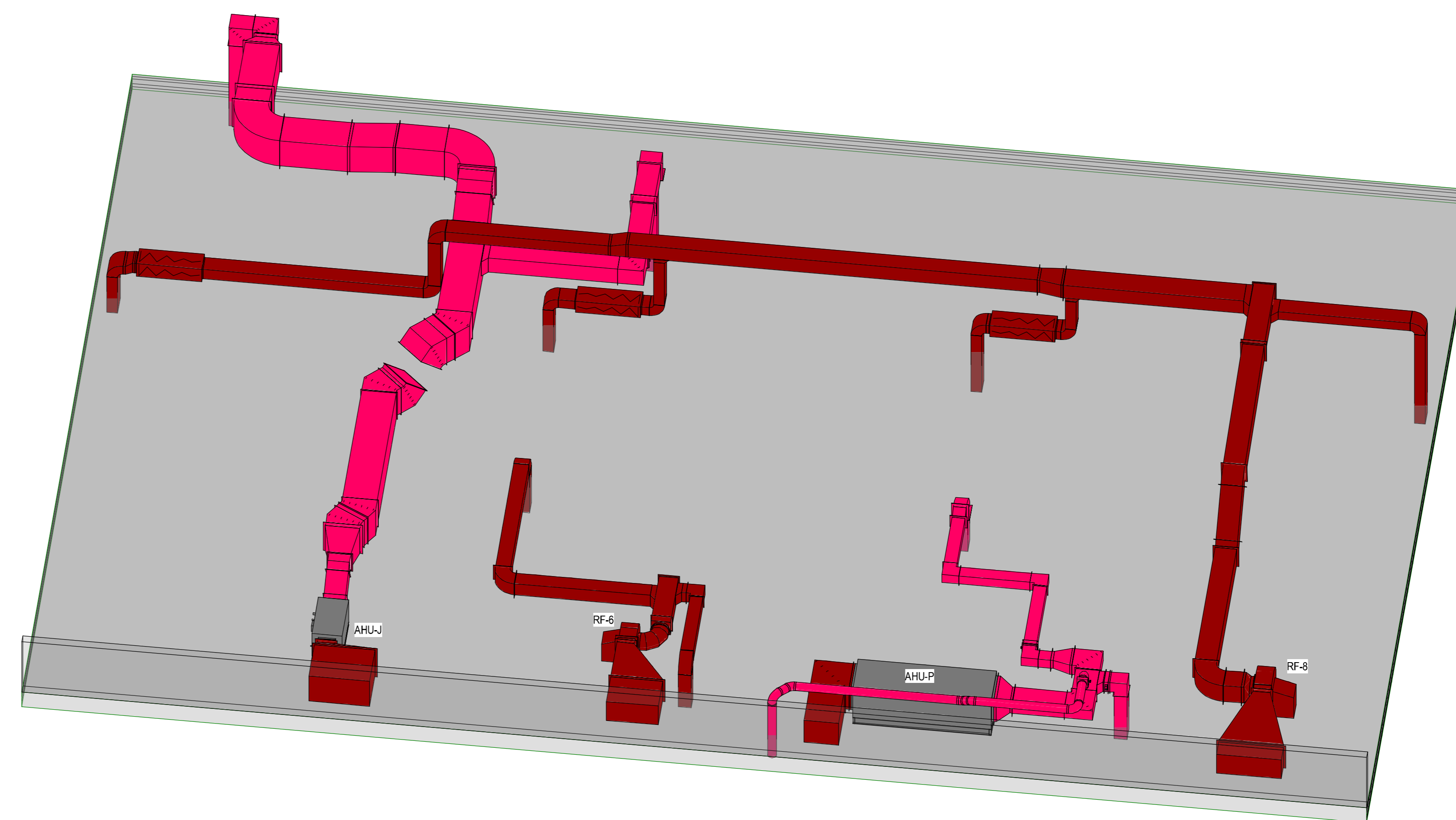
5 Plantroom View 5
